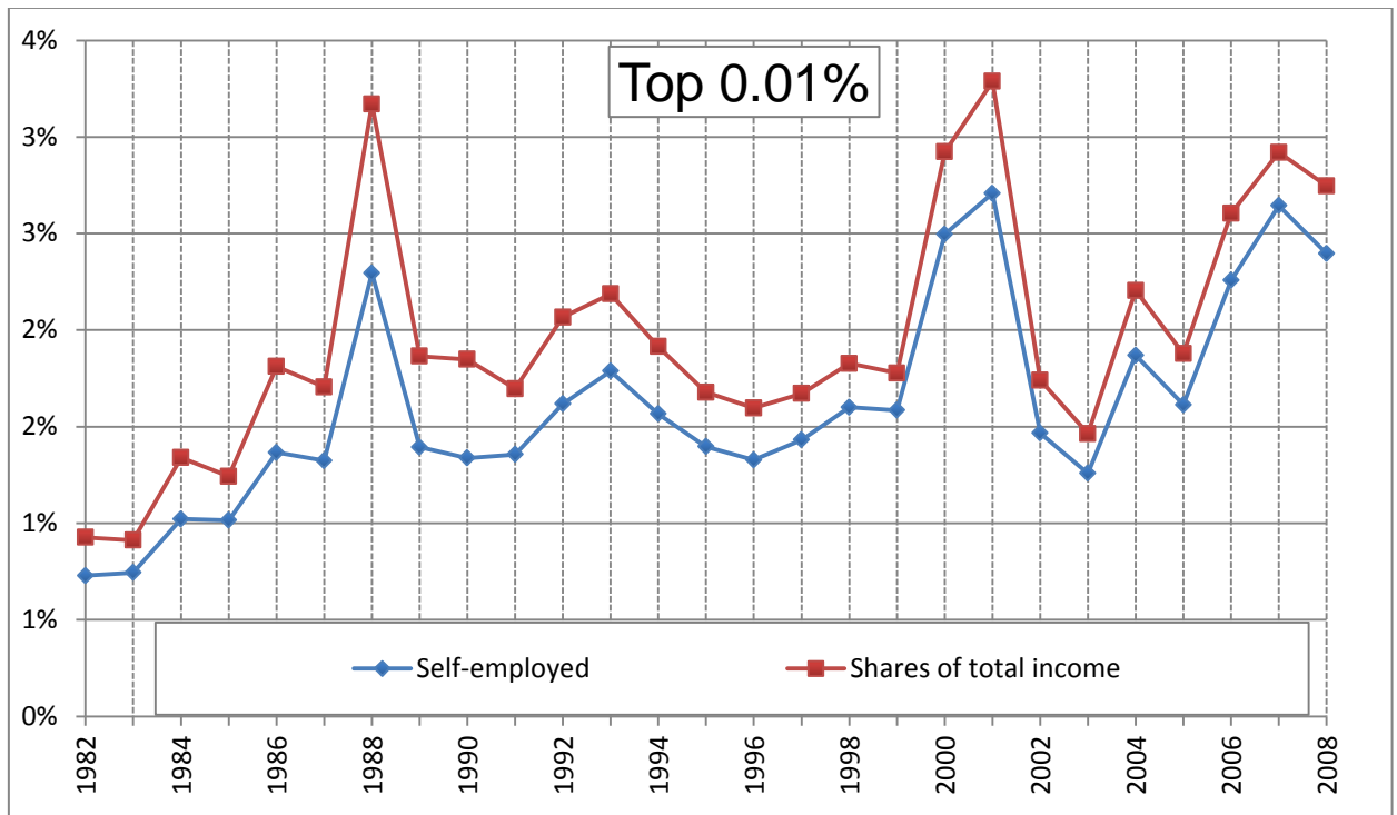
Figure 9.f) Top 0.01% share
